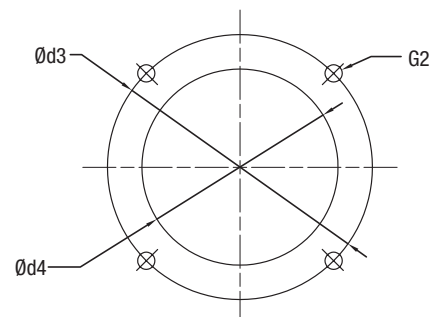
Mounting Detail
