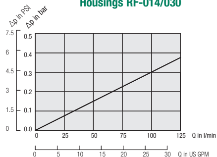
Housings RF-014/030
